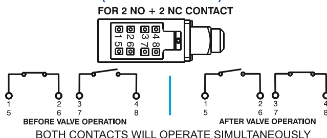
FIG. 3 : LIMIT SWITCH (COVER REMOVED) MODEL : T-6-LSM- 2 NO
