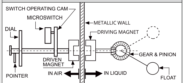
FIG. 2 FLOAT LEVEL
