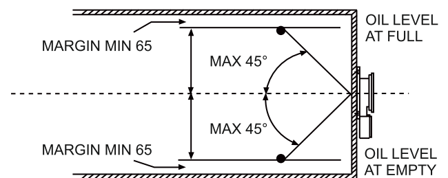
FIG. 2 FLOAT LEVEL
