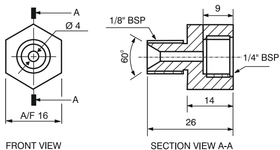
FIG. 2: CONNECTOR FEMALE-1/4" BSP TO MALE-1/8"S"BSP
