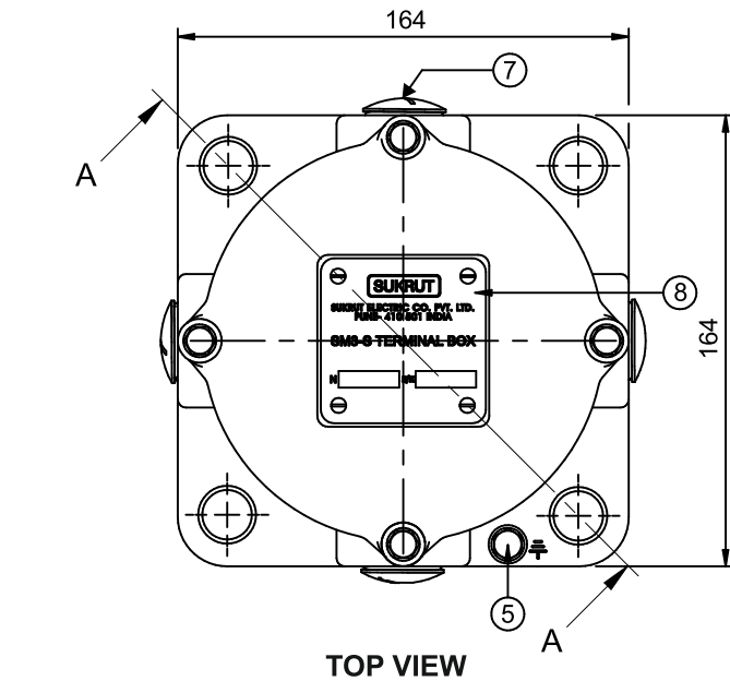
FIG 1. : CT TERMINAL BOX: SM3-S
