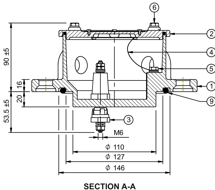
FIG 3. : TERMINAL POSITION
