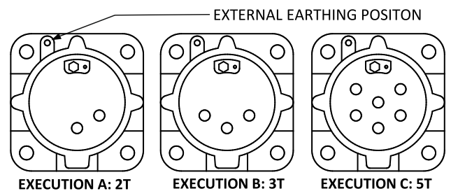
FIG 3. : TERMINAL POSITION
