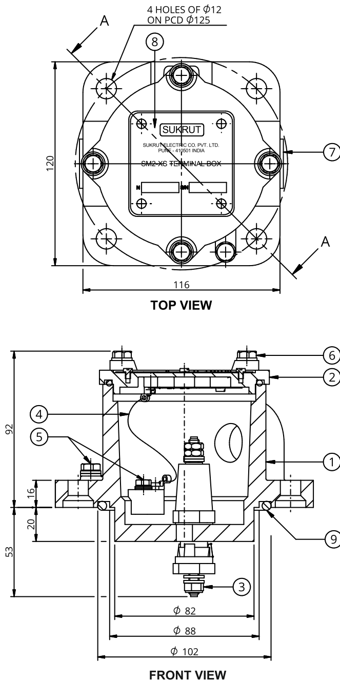
FIG 3. : TERMINAL POSITION
