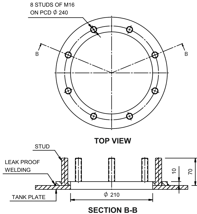
FIG 2. : MOUNTING PAD
