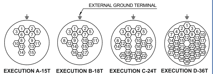
FIG 3. : TERMINAL POSITION
