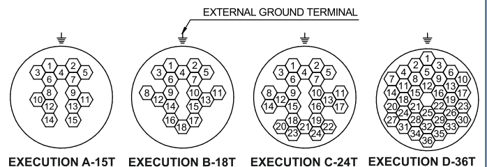
FIG 3. : TERMINAL POSITION
