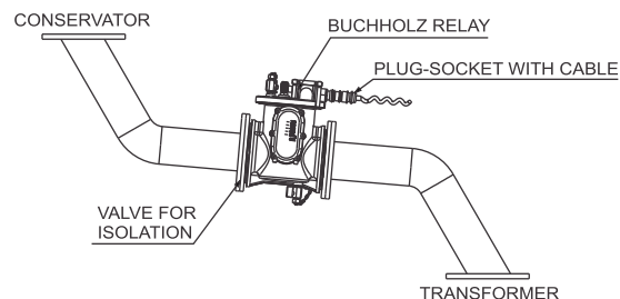
FIG 2. APPLICATION OF BUCHHOLZ RELAY
