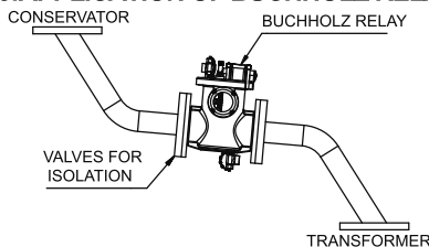
FIG 6.APPLICATION OF BUCHHOLZ RELAY
