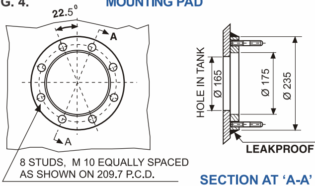
FIG. 4. MOUNTING PAD
