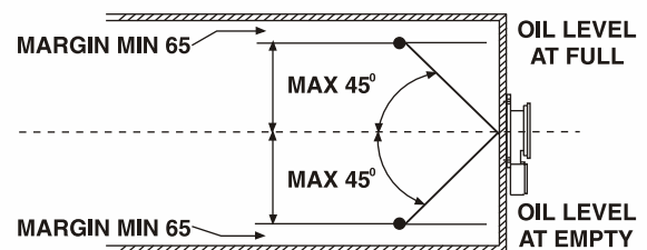
FIG. 2 FLOAT LEVEL
