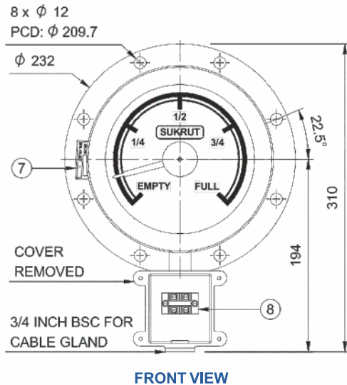
FIG 3. OIL LEVEL INDICATOR : SO-6-M
